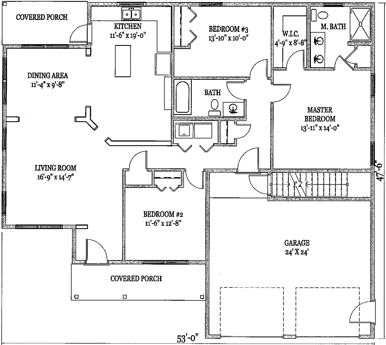
○ FIRST FLOOR PLAN N.T.S. 1,534 SQUARE FOOTAGE
