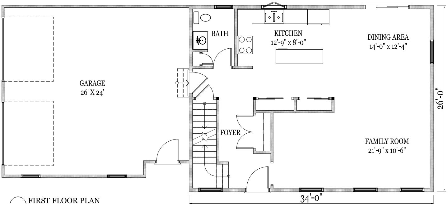
○ FIRST FLOOR PLAN N.T.S. 884 SQUARE FOOTAGE
