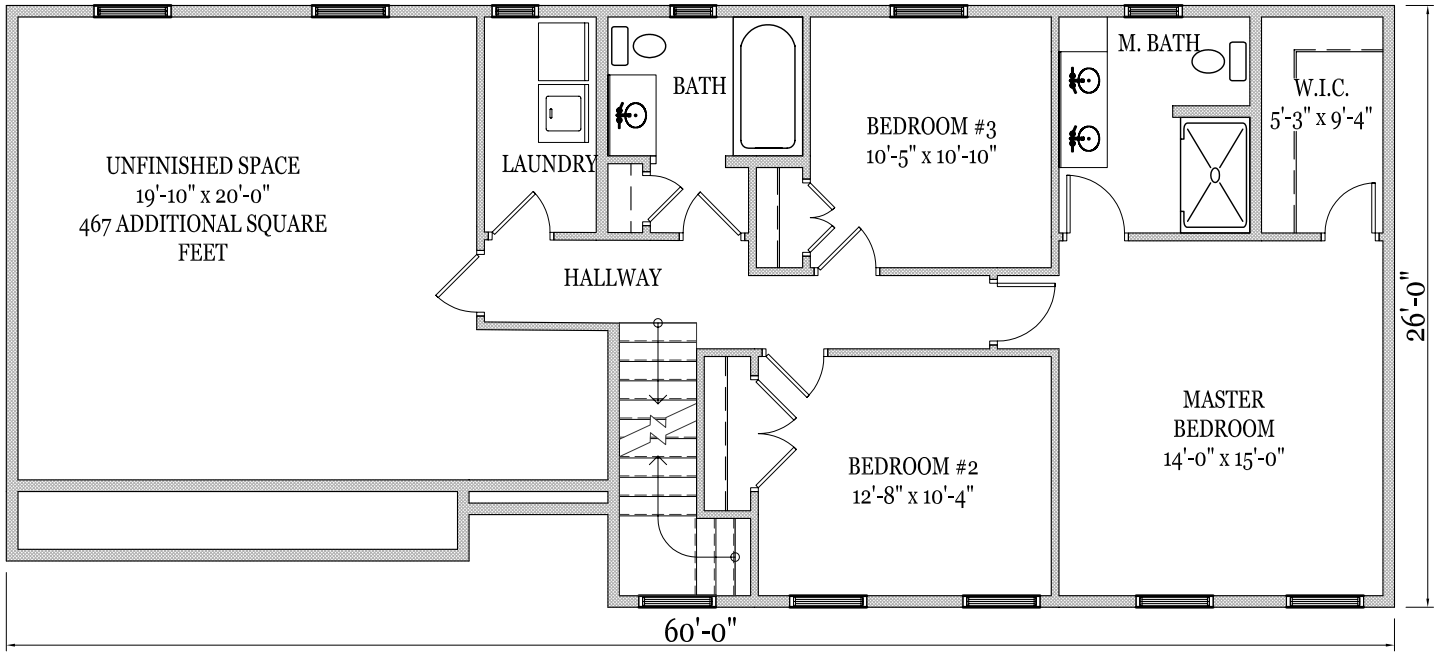
○ SECOND FLOOR PLAN N.T.S. 964 SQUARE FOOTAGE
